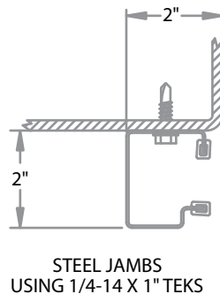
WOOD JAMBS USING 1/4" X 10 X 1" LAG CONCRETE/MASONRY JAMBS USING 1/4" X 1-3/4" WEDGE-BOLT
